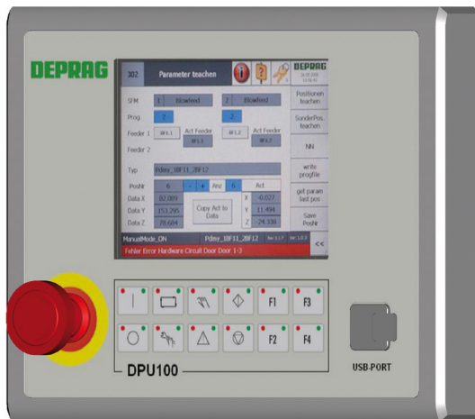
DEPRAG DPU100 – Controller- an all-in-one control unit that simplifies the control functions of all workstation components
