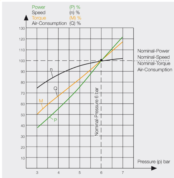
Speed regulation using the air-pressure
