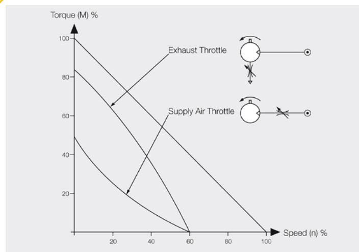
Speed regulation using the supply air
