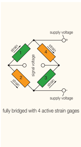
Function principle of the strain gage transducers
