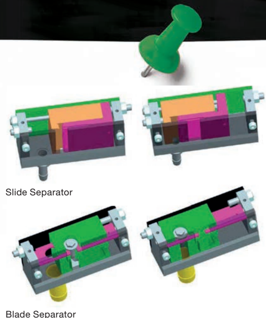
Image 7: In multiple feeding systems, the separator supplies the feed-components to the required positions.
