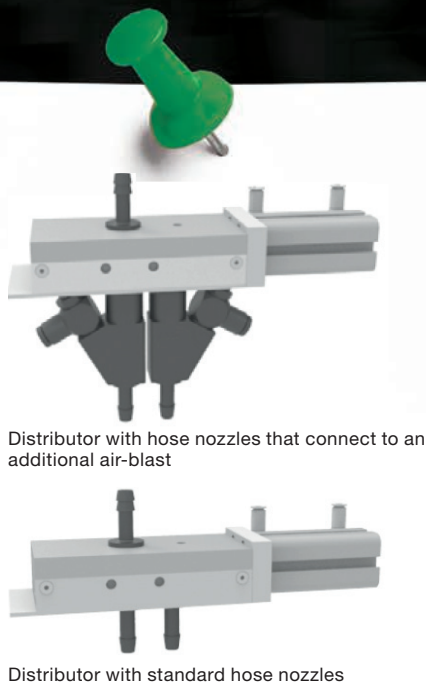
Image 6: Two distributor design examples.
