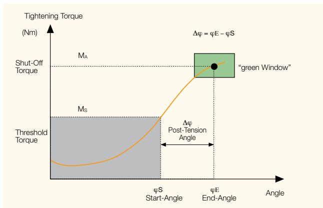
Angle-controlled tightening
