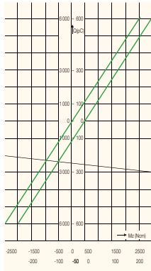
Linearity diagram
