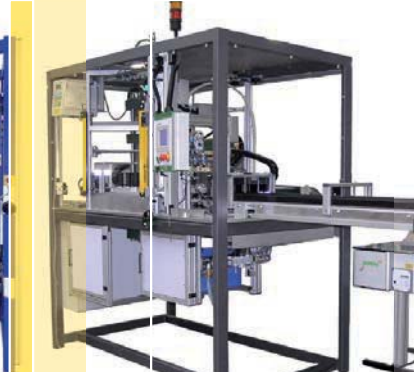
Screw assembly of anti-vibration handles
